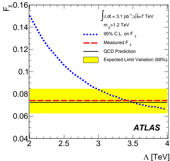
FIG. 3. The dashed horizontal line is the measured F_\chi (see text) and the solid horizontal line is the QCD prediction, with a band to illustrate a 1\sigma variation of the expected limit. The dotted curve is the 95% CL exclusion contour for F_\chi with quark contact interactions, used to set the exclusion limit on \Lambda .
