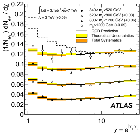
FIG. 1. The normalized \chi distributions for 340 < m_{jj} < 520 GeV, 520 < m_{jj} < 800 GeV, 800 < m_{jj} < 1200 GeV, and m_{jj} > 1200 GeV, with plotting offsets shown in parentheses. Shown are the QCD predictions with systematic uncertainties (bands), and data points with statistical uncertainties. The prediction for QCD with an added quark contact term with \Lambda = 3.0 TeV is shown for the highest mass bin m_{jj} > 1200 GeV.
