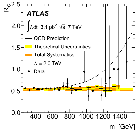
FIG. 2. Dijet centrality ratio, R_C , as a function of m_{jj} , with all events above a mass of 1400 GeV plotted in the last bin. Shown are the QCD prediction with systematic uncertainties (bands), and data points with statistical uncertainties. The prediction for QCD with an added quark contact term with \Lambda = 2.0 TeV is also shown.
