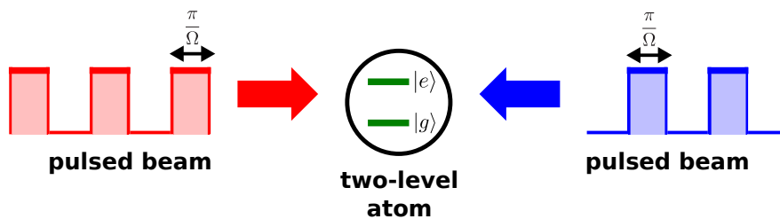
Figure 2.1: In the \pi -pulse model, the beams are described by discrete intensity pulses with duration \Delta t = \frac{\pi}{\Omega} . Each pulse drives half of a Rabi period and changes the state of the atom from ground to excited and vice versa. Coherent sequences of absorption from one side and stimulated emission from the other side exert a force on the atom, which exceeds the radiative limit, if \Omega \gg \gamma .
